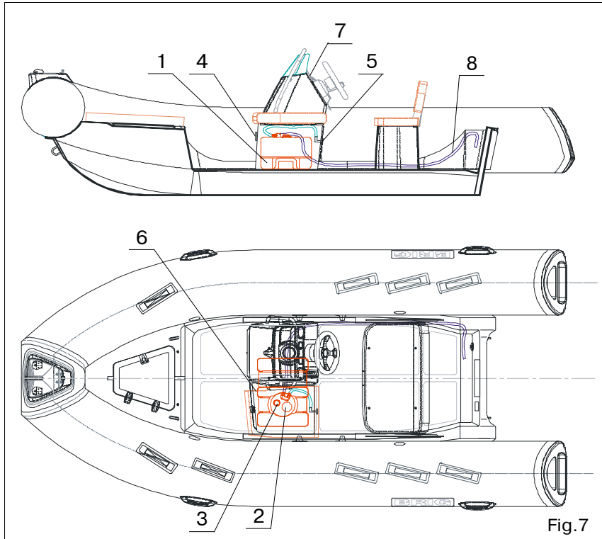
Fuel system for TENDER DELUXE version ( Fig.7).
