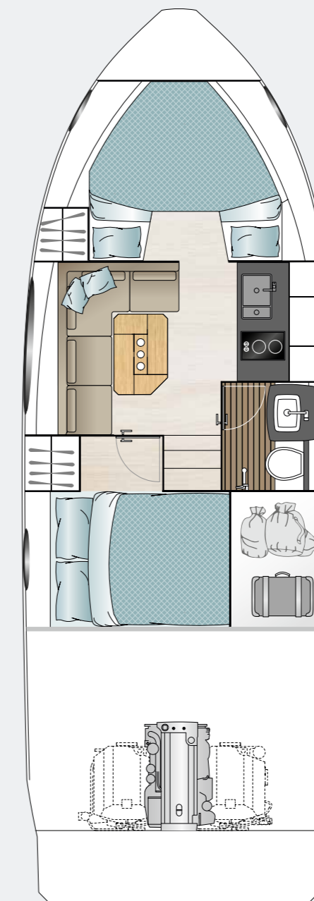
LOWER DECK
