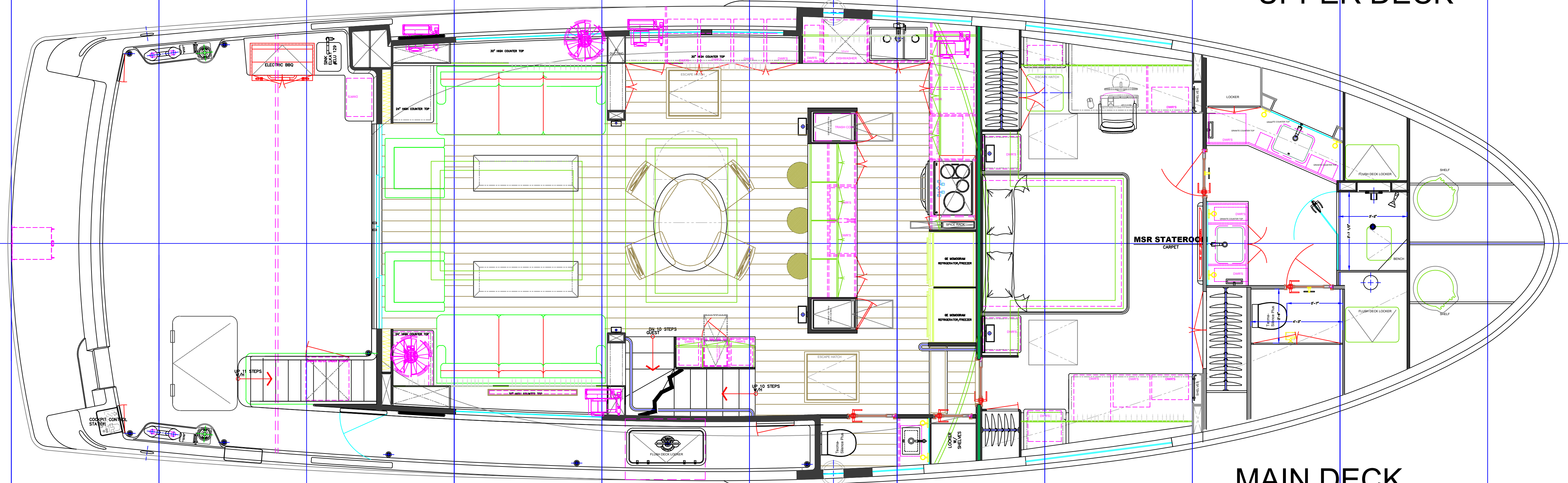
MAIN DECK
