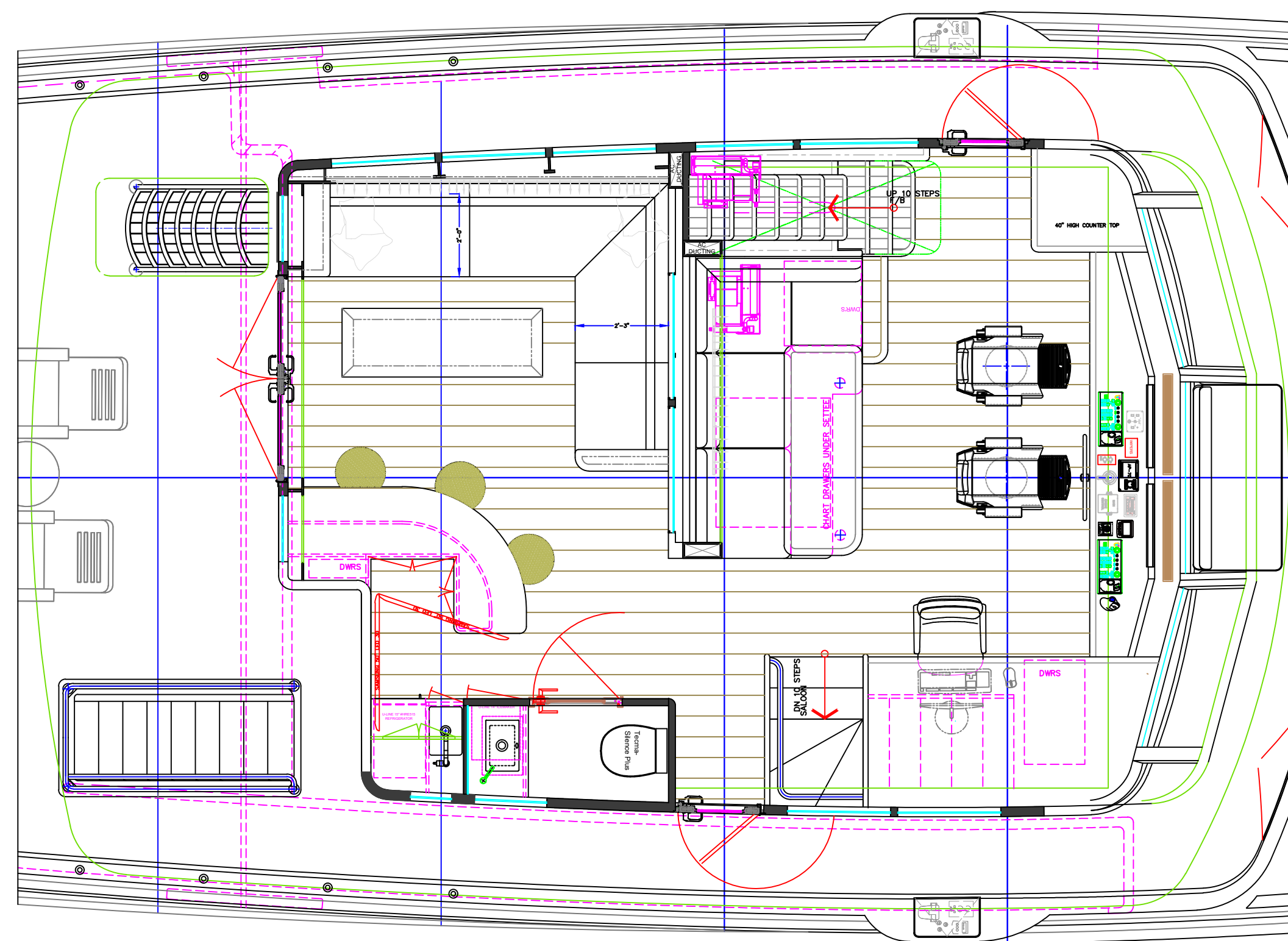
SKY LOUNGE LAYOUT
