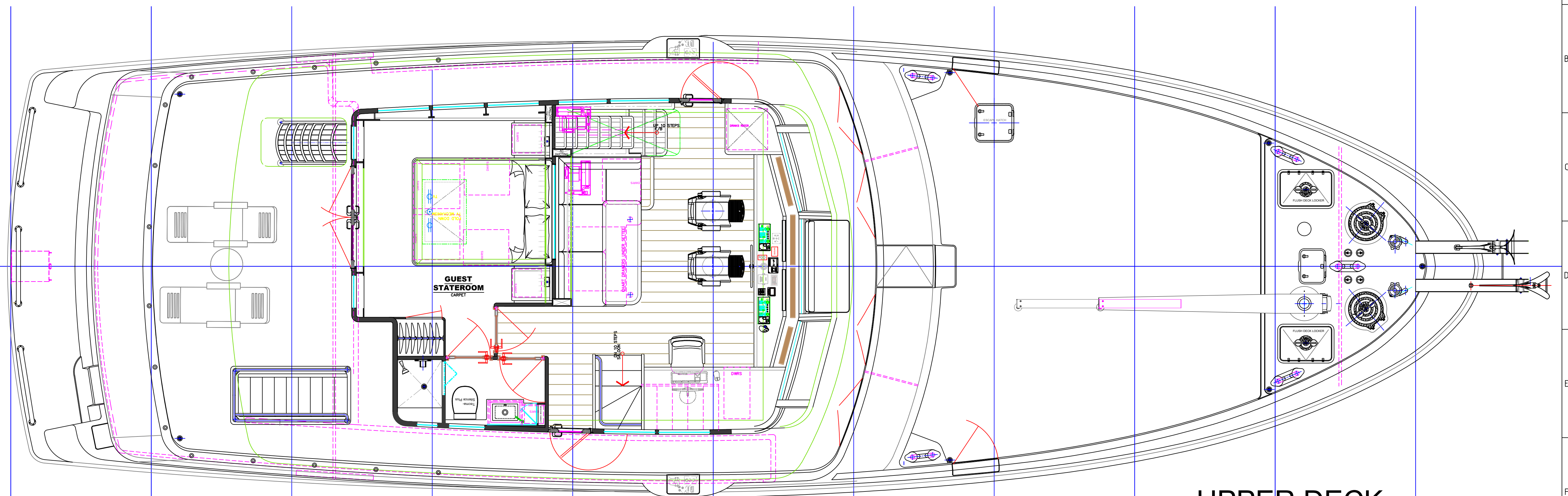
UPPER DECK
